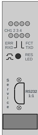
Figure 11: Front panel of the CD9234 with LEDs, button and service interface
