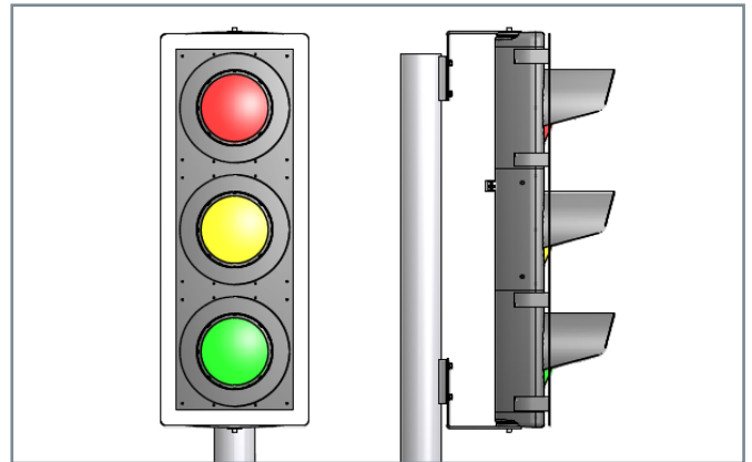
Picture Text: Technical drawings of the 3-aspect RAG FUTURA UK signal head
