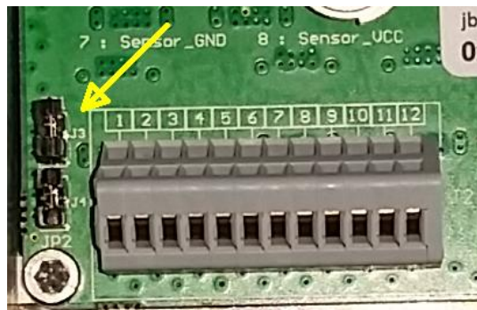
Figure 6: J3 and J4 determine RS485 full/half duplex operation
